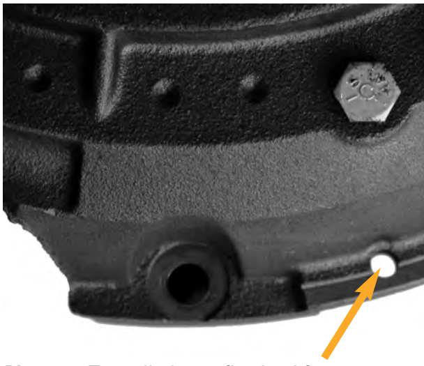
Picture 1: Tap roll pins to flywheel face
