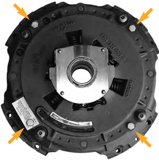
Picture 1: Remove four yellow bolts
